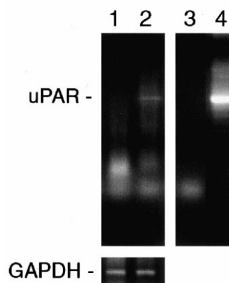
Fig. 4. uPA increases uPAR mRNA in thyroid cells. TAD-2 cells were incubated with (lane 1) or without (lane 2) 5 nM DFP-uPA for 24 h. PCR was performed with 1 \mu l of reverse transcribed cDNA (lanes 1, 2) or without DNA as negative control (lane 3) in the presence of primers for uPAR or for GAPDH. 10 ng of uPAR cDNA was amplified as a positive control (lane 4). PCR products were analyzed by 1% agarose gel containing ethidium bromide, followed by photography under ultraviolet illumination.
